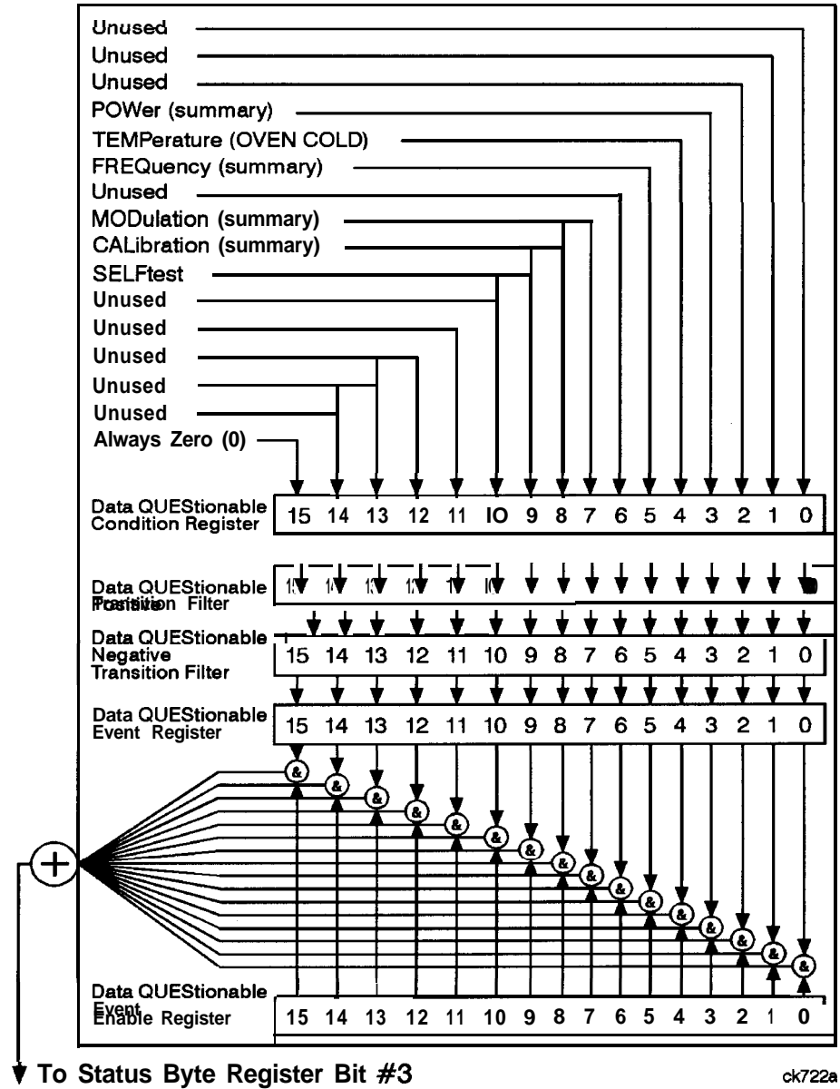
Figure 2-19. The Data Questionable Status Group
