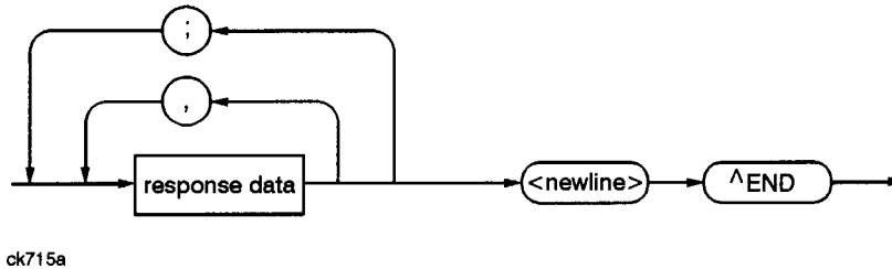
ck715a Figure 2-14. Simplified Response Message Syntax
