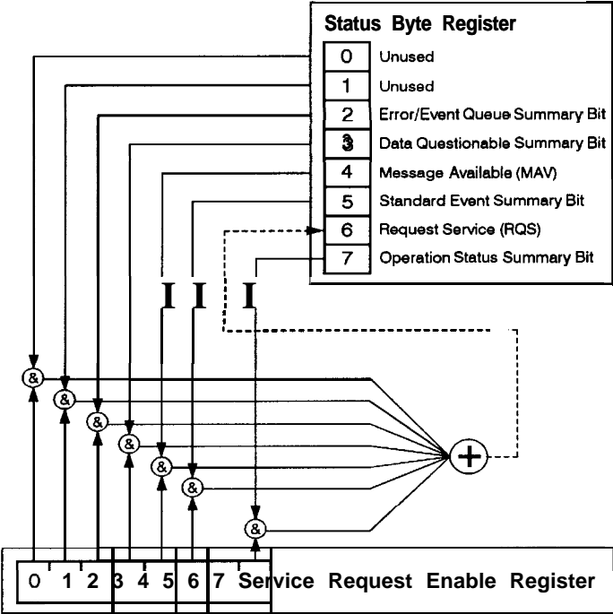
Figure 2-16. The Status Byte Group
